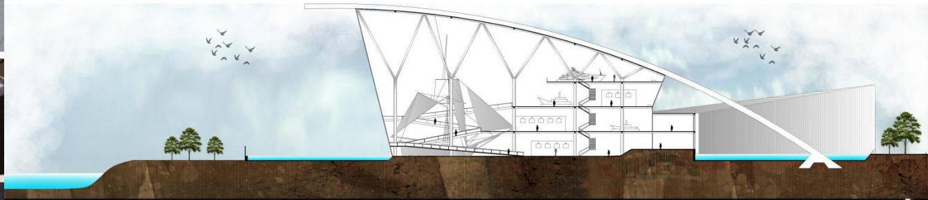
Section BB
